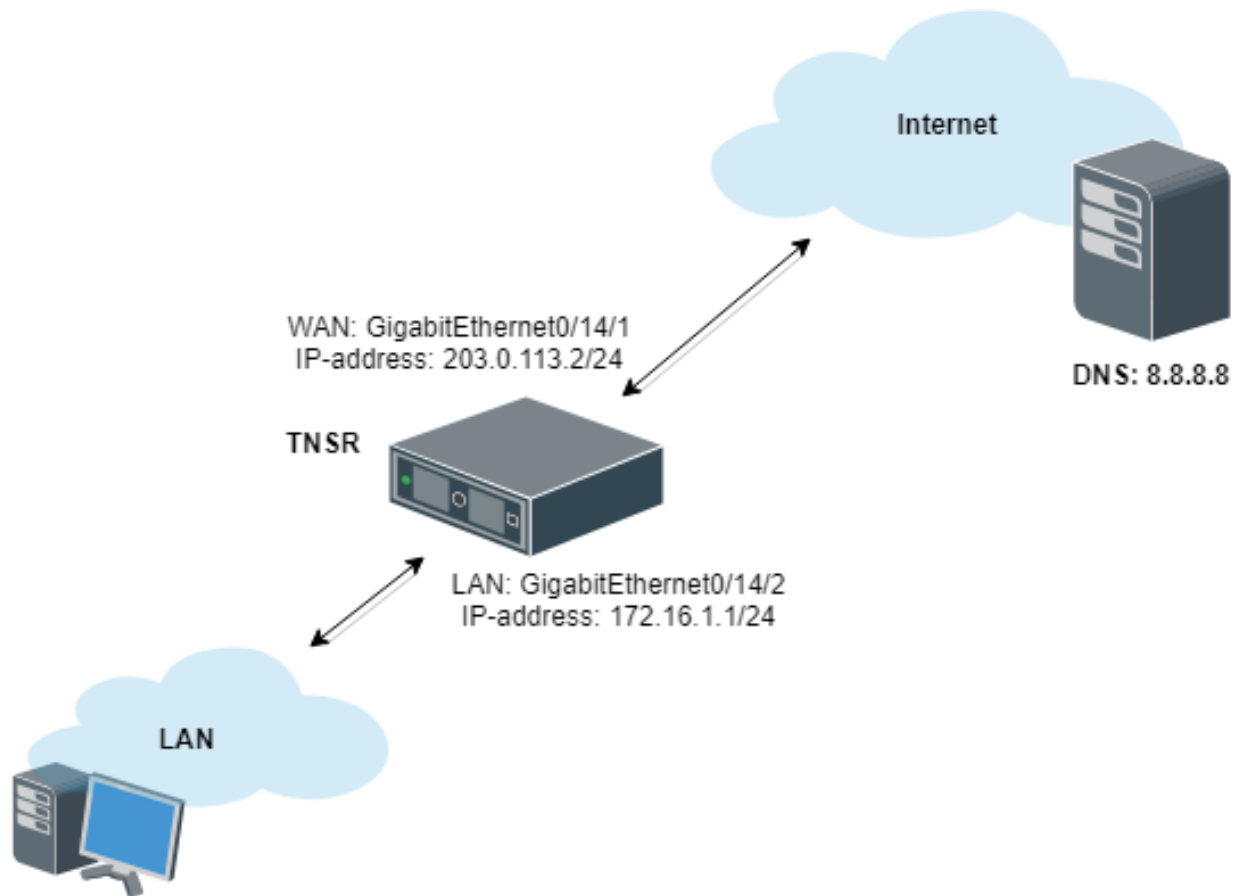
Fig. 5: Basic SOHO Router Example
