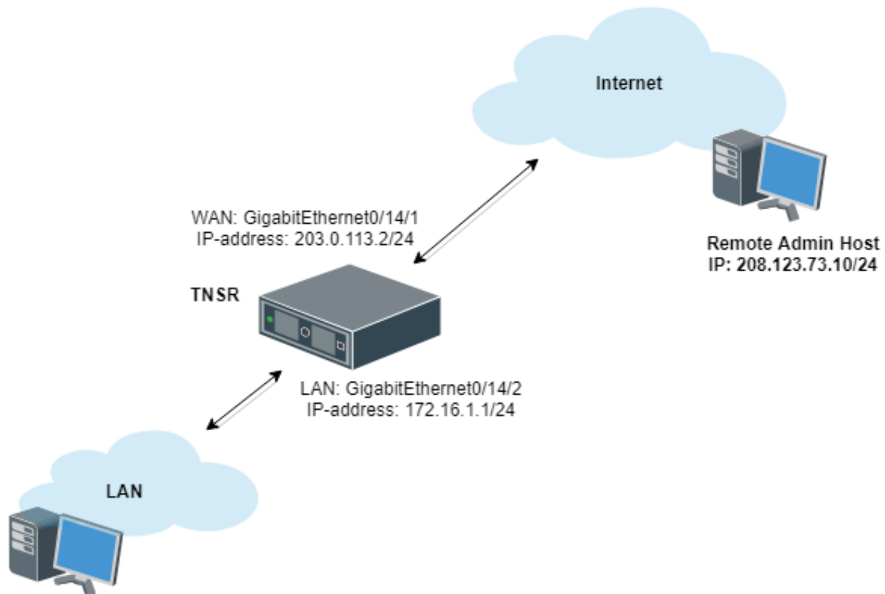
Fig. 6: ACL Example Scenario
