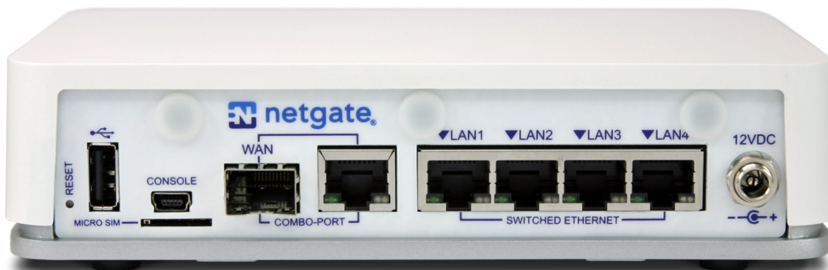
Fig. 1: Rear view of the Netgate 2100 Firewall Appliance The items in this image are described by entries in Routed Ethernet , Switched Ethernet , and Other Ports .
